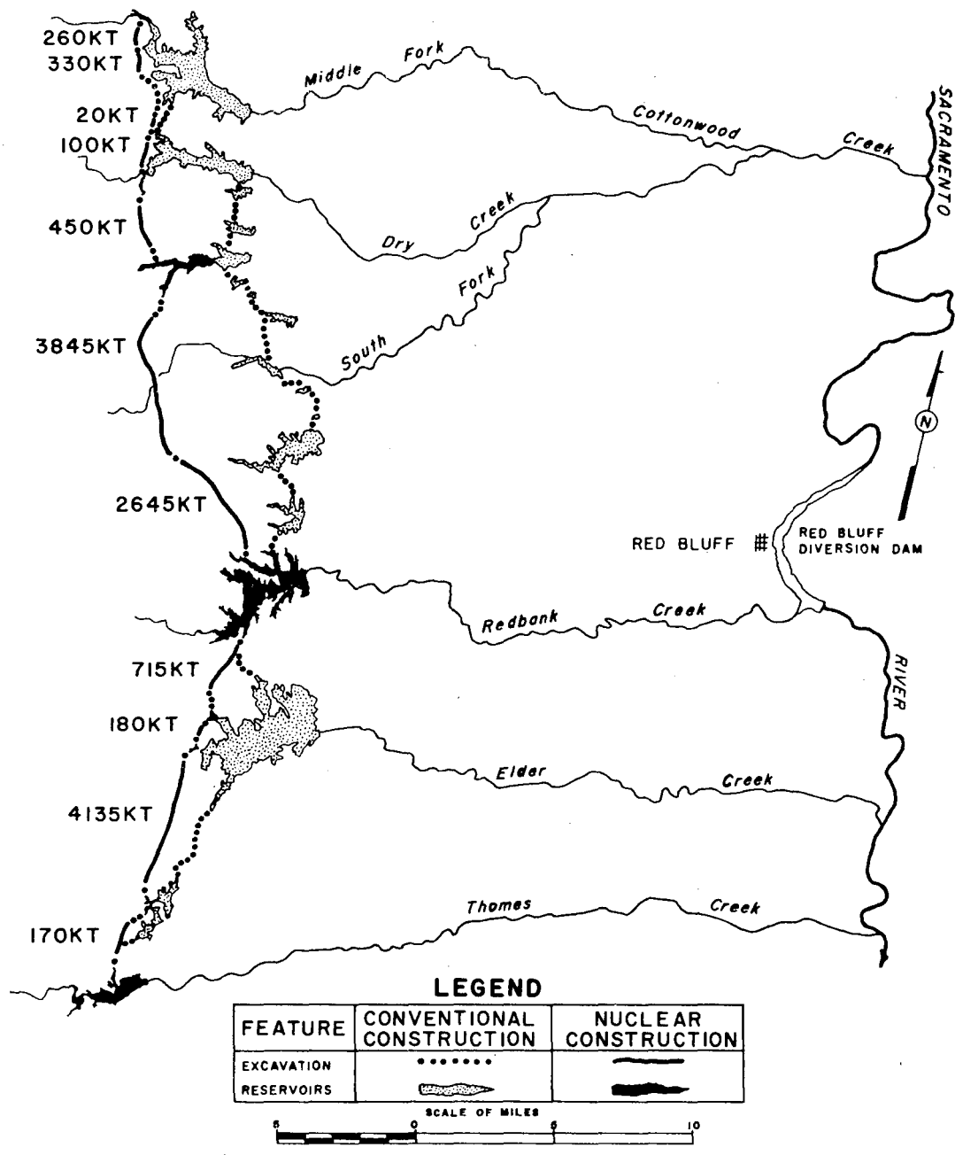
Fig. 2. Alternative alignments - West Side conveyance system.
